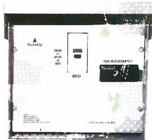
INSIDE PANEL VIEW (accessible without the use of tools)
